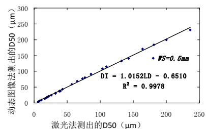
(a) WS=0.5mm
