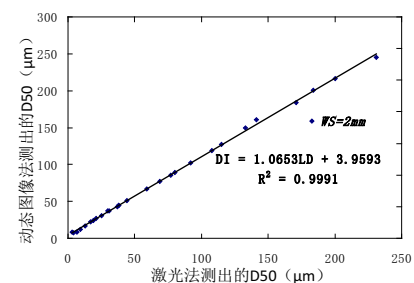
(b) WS=2mm
